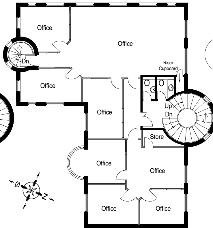
First Floor. Net internal area (sq ft): 1687
